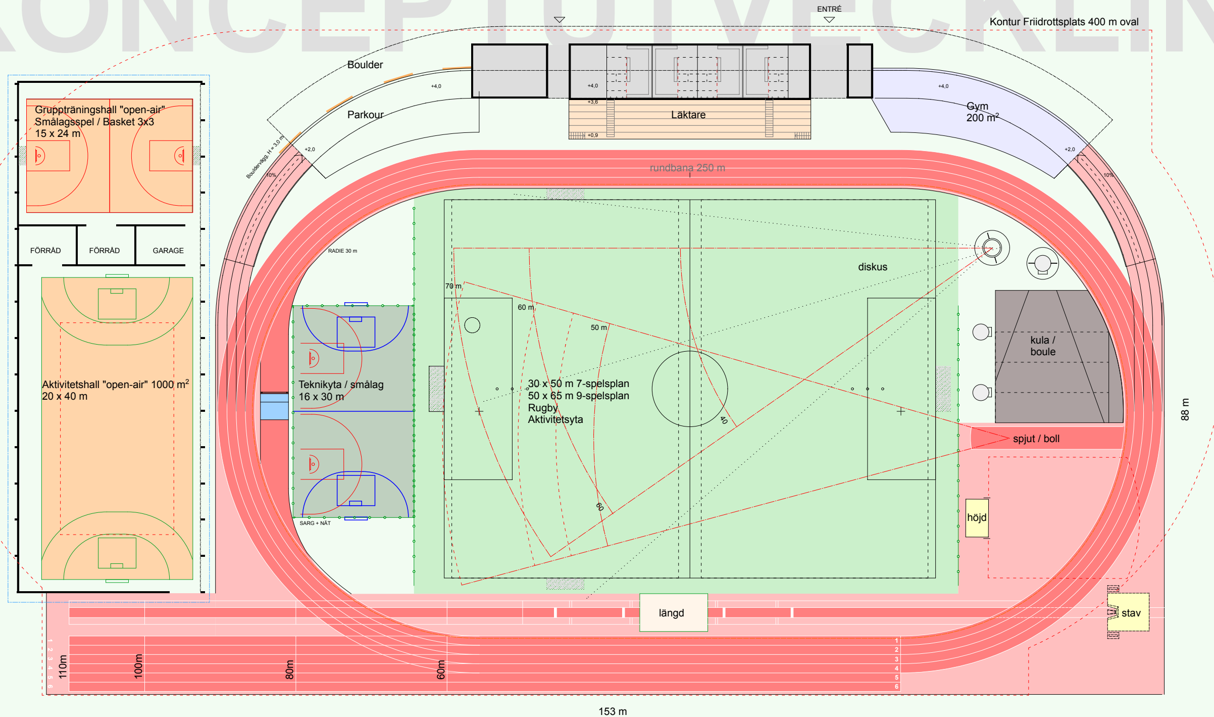
LAYOUT PLAN 1 SKALA 1:500
